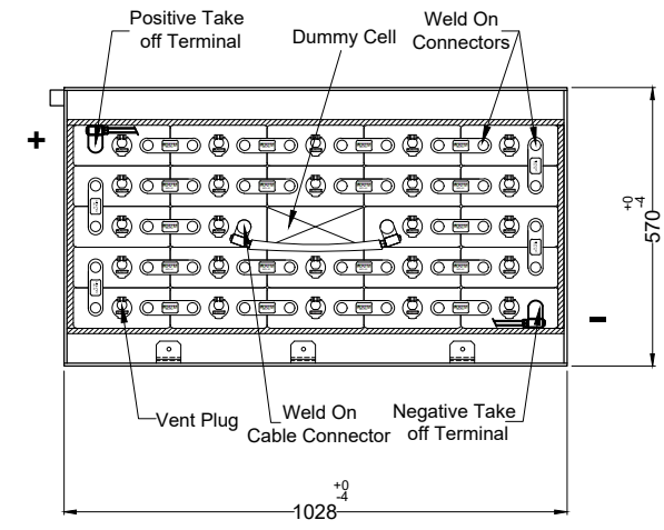
CONNECTION LAYOUT FOR 48V 560Ah
