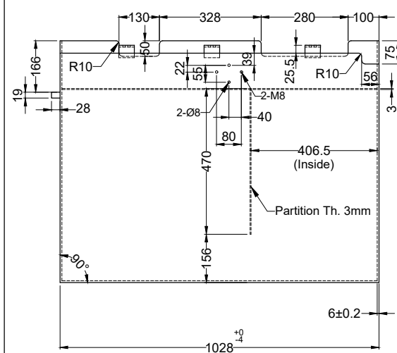
TRAY FOR 48V 560Ah
