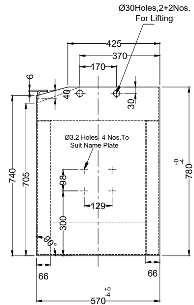
TRAY FOR 48V 560Ah
