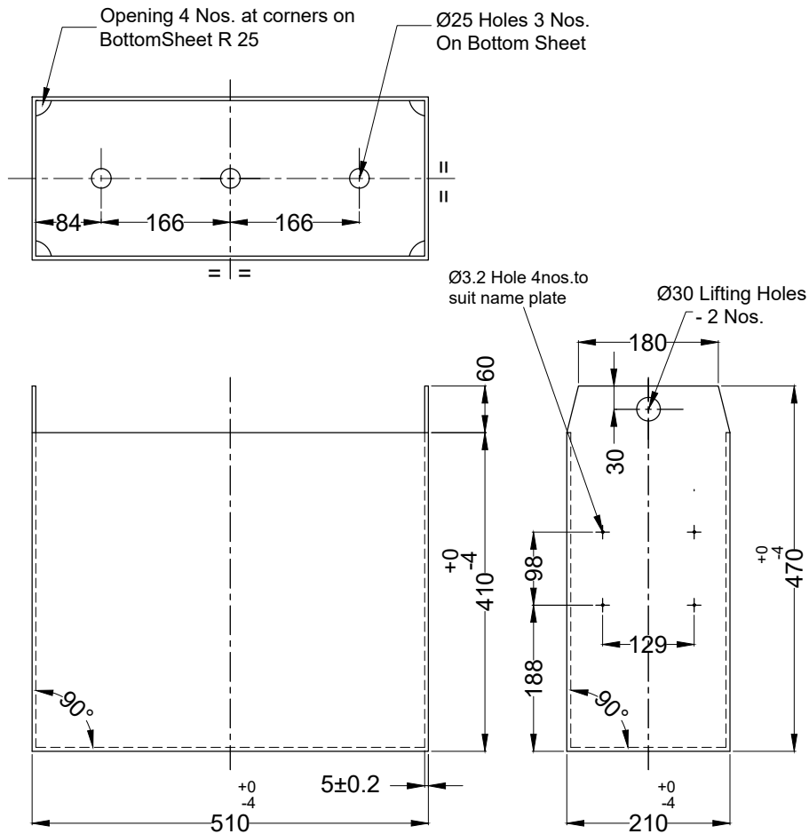
TRAY FOR 12V 320Ah
