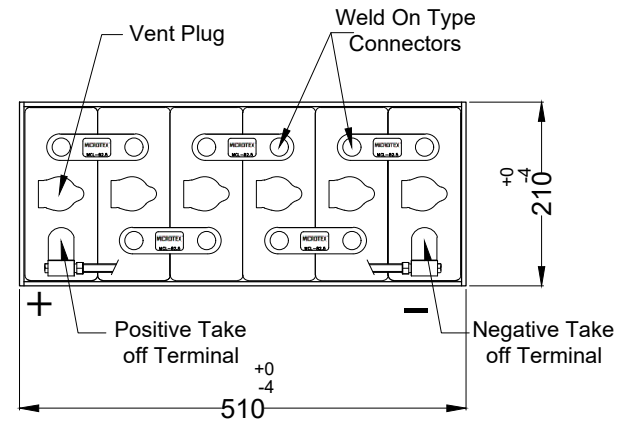
CONNECTION LAYOUT FOR 12V 320Ah
